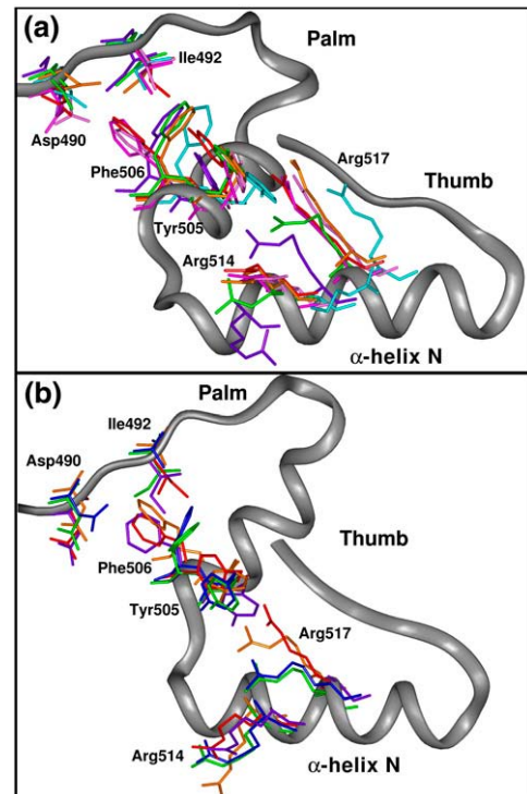
FIGURE 3 Residue side-chain orientations in the crystal binary (PDB entry 1XSL, green) and ternary (PDB entry 1XSN, red) pol- \lambda complexes as well as in all simulations performed. ( a ) Positions of key residues in crystal binary and ternary states and in all simulations of wild-type pol \lambda after 20 ns. Simulations 1 (purple), 2 (cyan), 3 (magenta), 4 (pink), and 5 (orange); see Table 2. ( b ) Positions of key residues in crystal binary and ternary states and in all simulations of mutated forms of pol \lambda after 20 ns. Simulations 6 (blue), 7 (orange), and 8 (purple); see Table 2.
