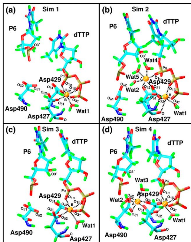
FIGURE 4 Active site arrangements from all simulations of wild-type pol \lambda with substrate (dTTP) present (Simulations 1–4, Table 2). The coordinations of the catalytic Mg 2+ ion ( A ) and nucleotide-binding Mg 2+ ion ( B ) with surrounding atoms are depicted by the dashed lines. Water molecules are included.
