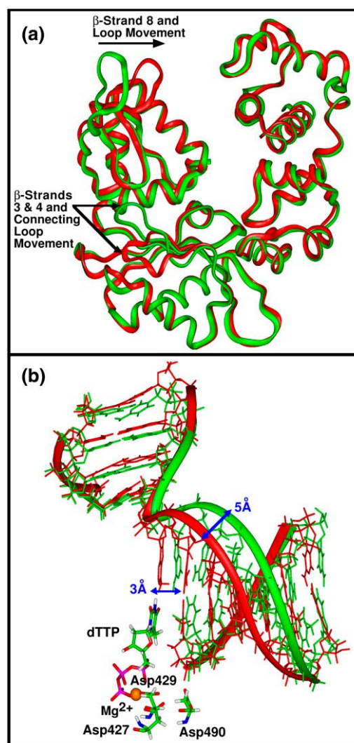
FIGURE 1 X-ray crystal binary (PDB entry 1XSL, green) and ternary (PDB entry 1XSN, red) pol \lambda /DNA complexes. (a) Superimposed C_{\alpha} trace of x-ray crystal binary and ternary pol- \lambda complexes. Differences between the x-ray crystal structures in the thumb and palm subdomains are shown by the arrows. (b) Position of the DNA template strand and templating base at the gap in the x-ray crystal binary and ternary structures of pol \lambda . The incoming nucleotide (dTTP) and active-site residues Asp 427 , Asp 429 , and Asp 490 of the ternary x-ray crystal structure are also shown. Key distances between the crystal binary and ternary states are provided and hydrogens are omitted from the DNA for clarity.
