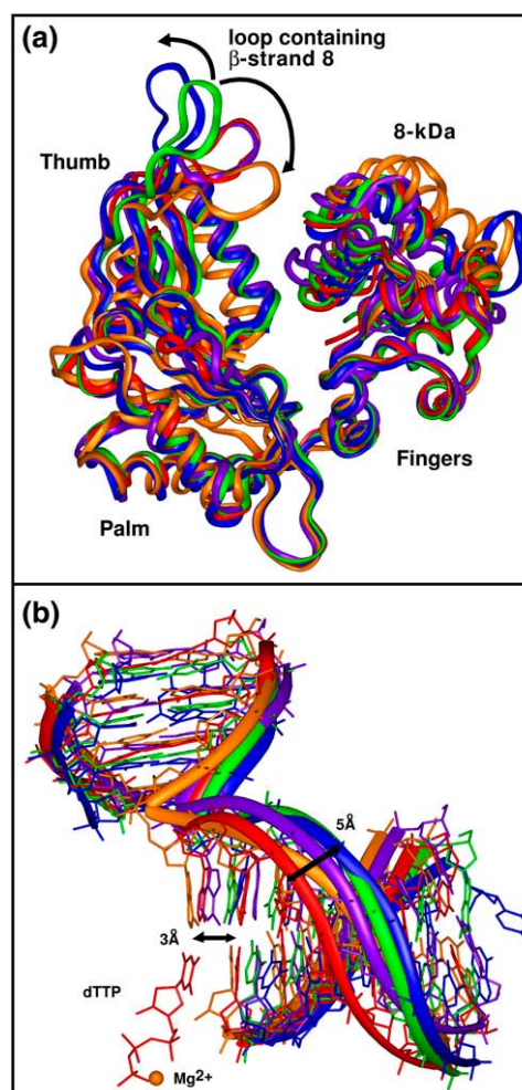
FIGURE 5 Subdomain and DNA motion in mutant DNA pol \lambda simulations. Simulations 6 (blue), 7 (orange), and 8 (purple), Table 2. (a) Subdomain motion in mutant simulations of DNA pol \lambda . All simulated mutated forms of pol \lambda are shown after 20 ns, superimposed along the C \alpha trace with crystal binary (PDB entry 1XSL, green) and ternary (PDB entry 1XSN, red) structures. Only residues 323–575 are shown for clarity. Arrows represent thumb loop motion from the initial binary conformation in Simulations 6 and 7. (b) DNA position in the crystal binary (PDB entry 1XSL, green) and ternary (PDB entry 1XSN, red) states as well as the DNA positions in all simulations of mutated forms of pol \lambda after 20 ns. Key distances between crystal binary and ternary states are also provided. Only the crystal ternary dTTP and Mg 2+ are shown. Hydrogens have been removed from all simulated structures for clarity.
